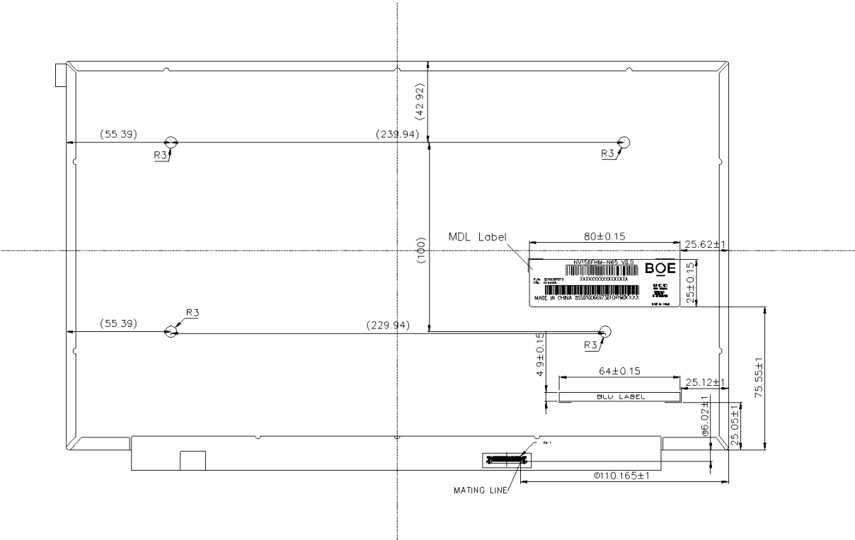
Figure 22. TFT-LCD Module Outline Dimensions (Rear view)
